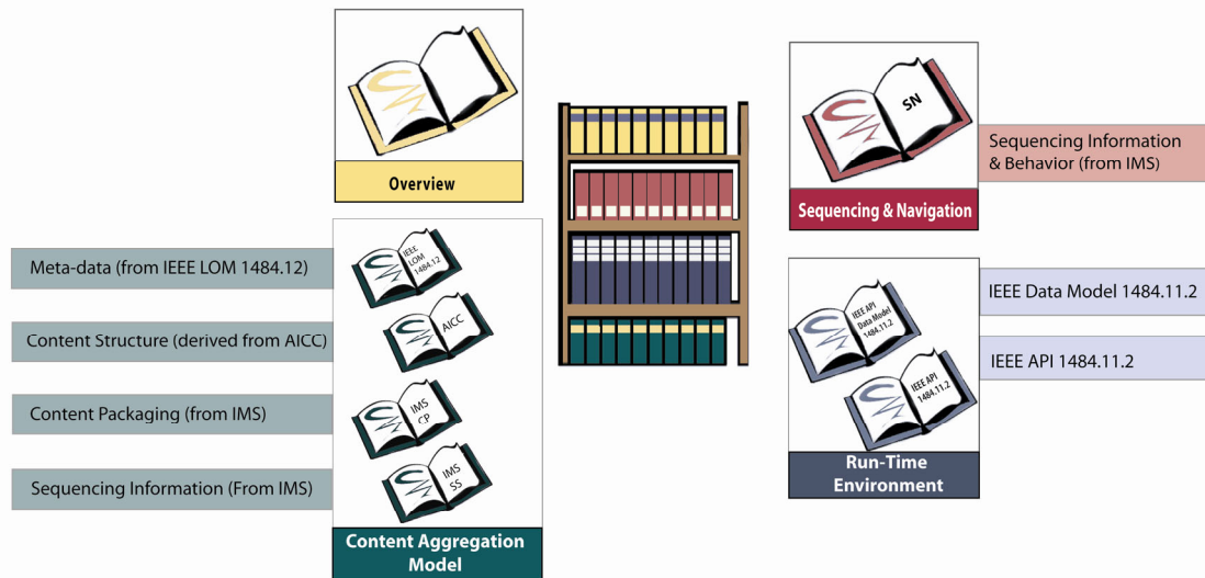
Figure 1.3.1a: SCORM Bookshelf
